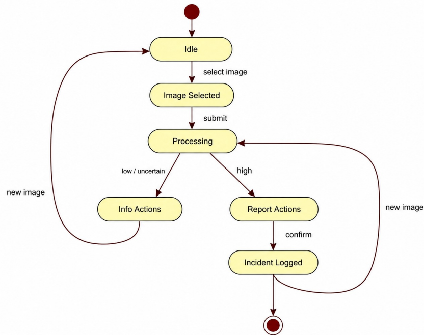
Figure 3.6: State transition diagram
